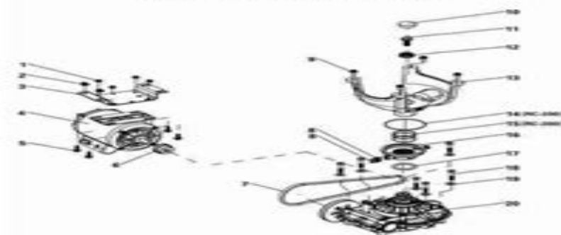
Shaft Housing Assembly
