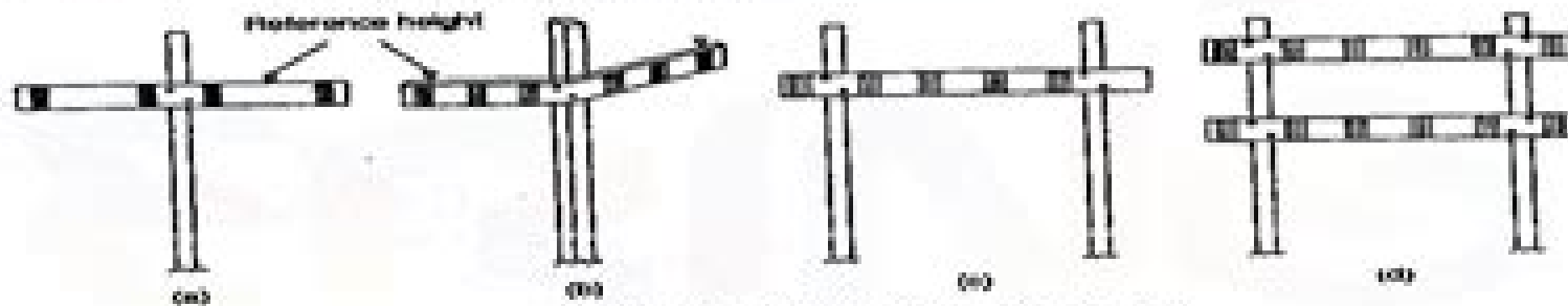
FIG. 20.7. VARIOUS FORMS OF SIGHT RAILS.
