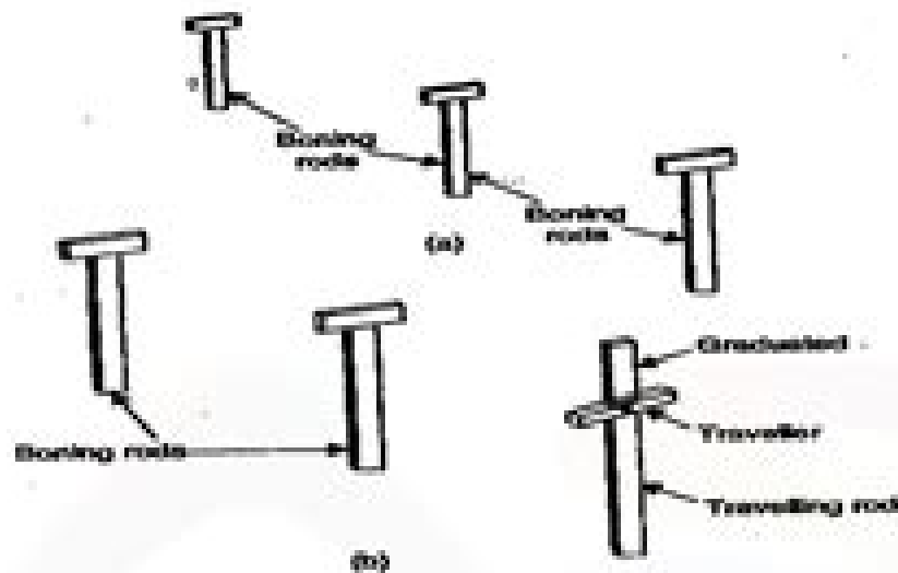
FIG. 20.5. (a) THREE BONING RODS. (b) TWO BONING RODS WITH A TRAVELLING ROD.
