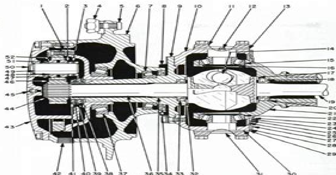
Fig. 024 — Cross sectional view showing components of front drive axle outer end.
