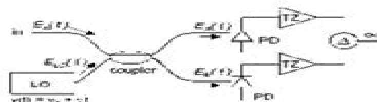
Fig. 1. Simplified block diagram of coherent optical spectrum analyzer. PD: Photodetector; T2: Transimpedance amplifier; LO: Optical local oscillator.
