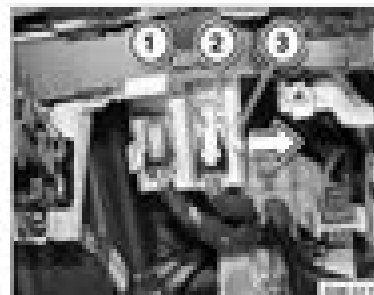
Fig. 10: Pull Leg (2) In Direction Of Arrow And Pull Out Control Unit Courtesy of BMW OF NORTH AMERICA, INC.
