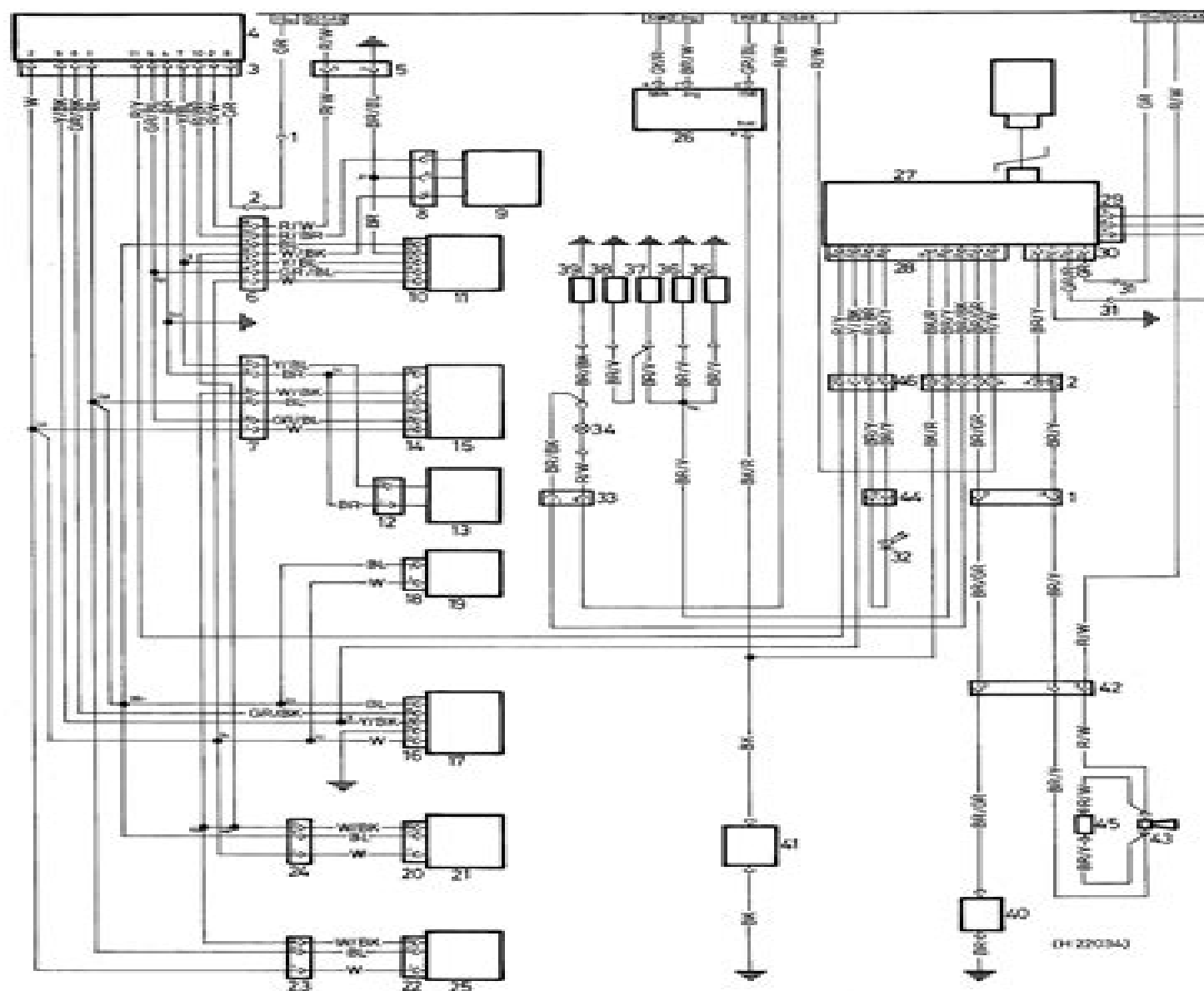
Typical wiring diagram for the central locking, burglar alarm, on-board computer, additional heater and digital clock (1 of 2)
