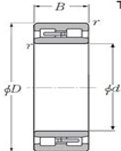
Cylindrical bore
