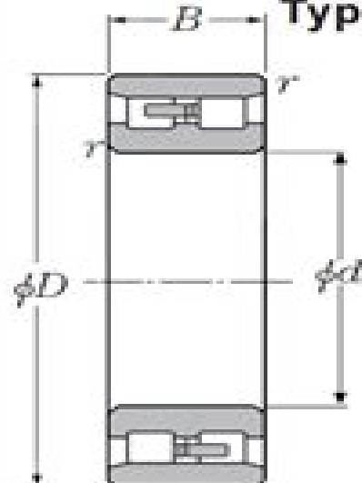
Cylindrical bore
