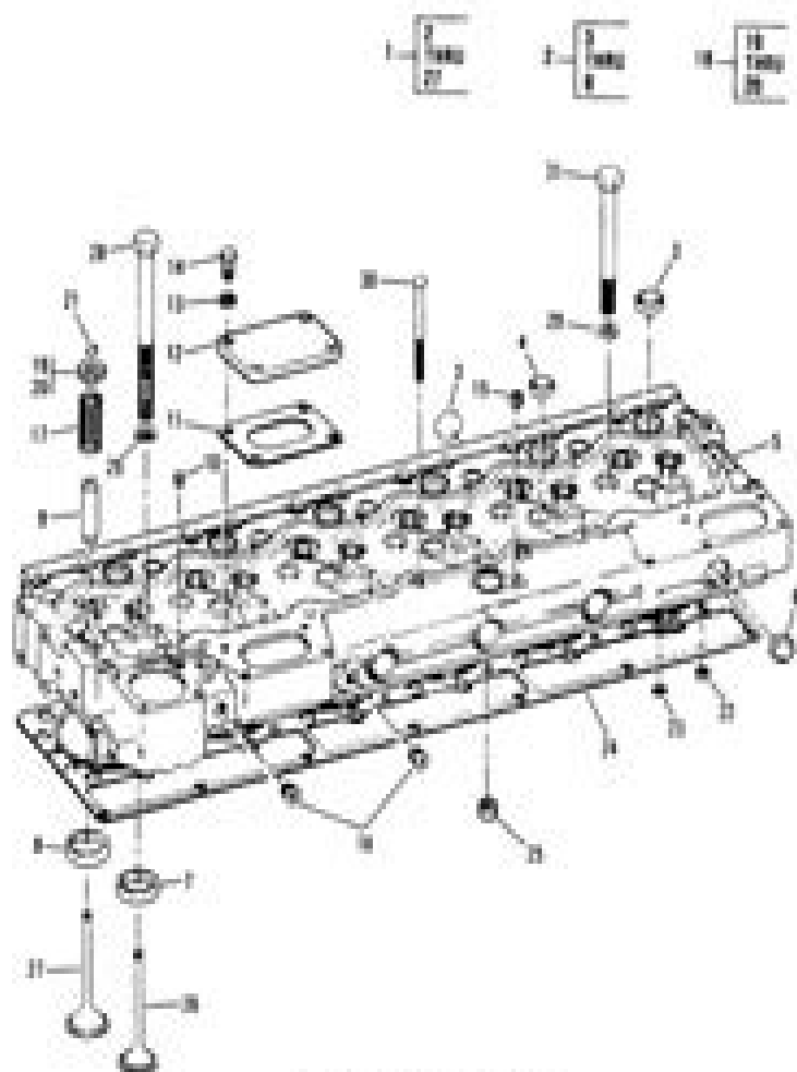
Figure 4. Cylinder Head Group
