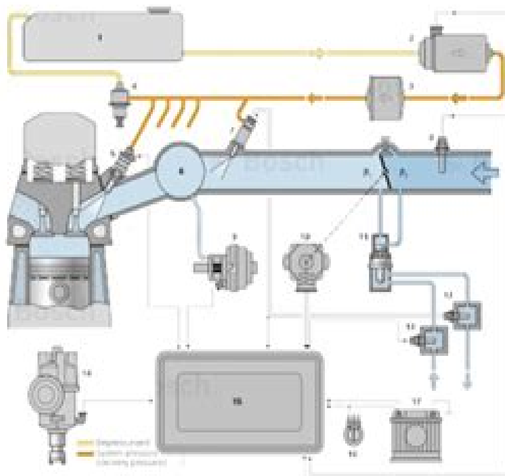
D-Jetronic system overview
