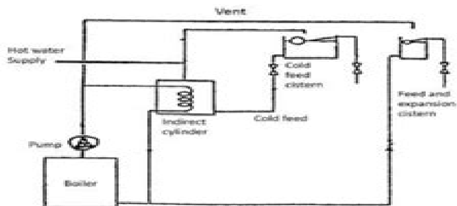
Figure 10 - Indirect hot water system.
