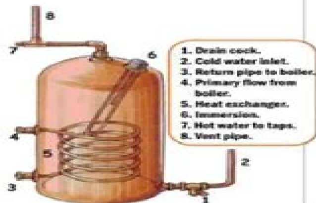
Figure 11 - Indirect cylinder.
