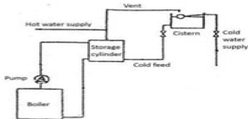
Figure 8 - Direct hot water system.
