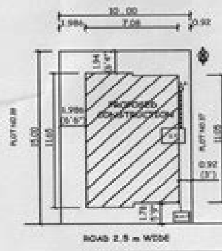
SITE PLAN
