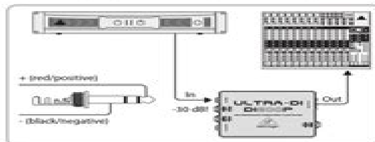
Fig. 3: Connection to a power amp output
