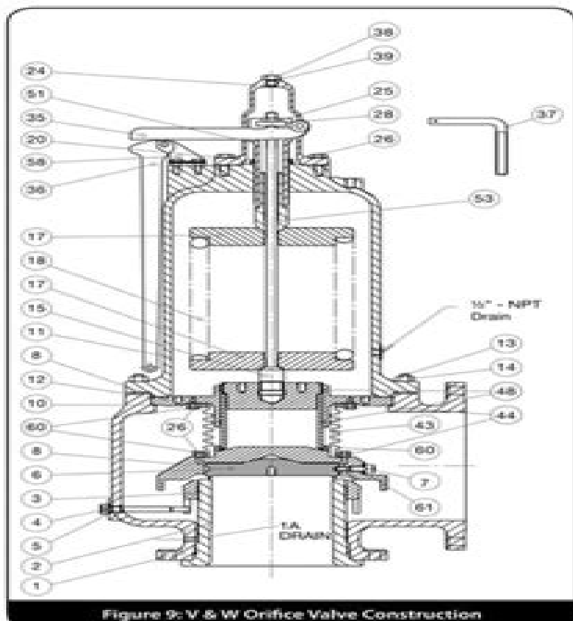
Figure 9: V & W Orifice Valve Construction
