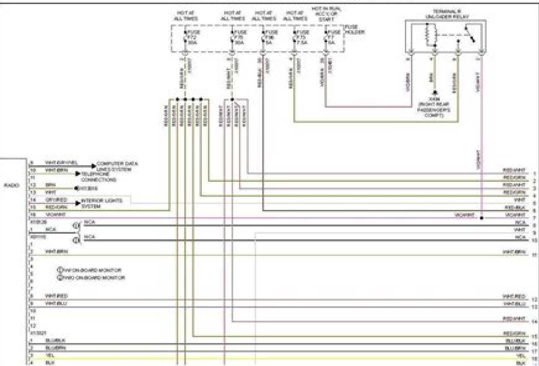
2005 BMW X5-Fig. 115: Premium Radio Circuit, W/ Top BIFT Radio (1 of 3)
