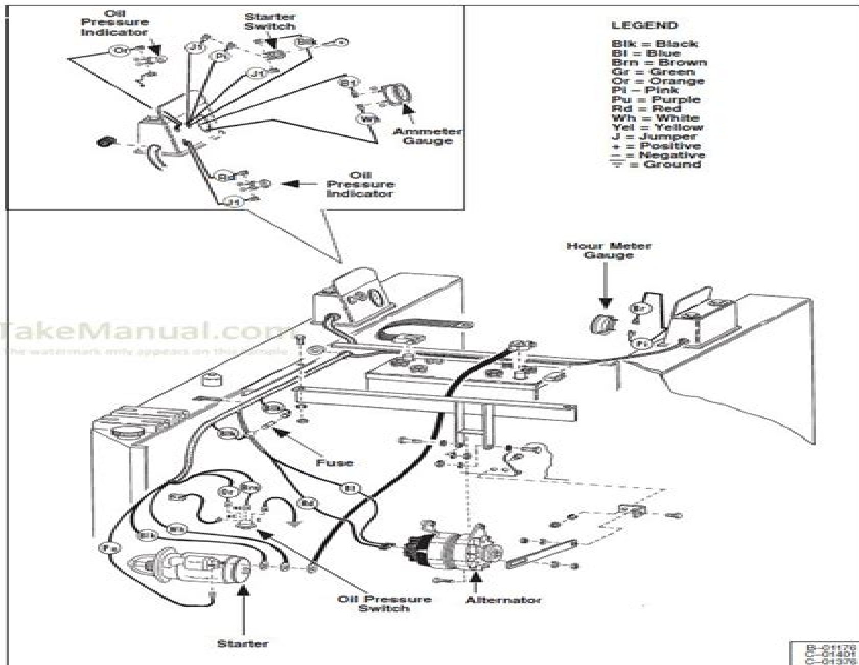
Fig. 1-56 Electrical Circuitry (Petter W/Lucas Alternators) (Added 1-2-76)
