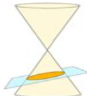
Ellipse
