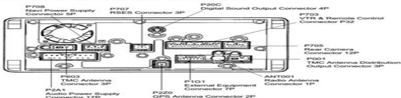
17 pin Honda Head Unit Audio connector
