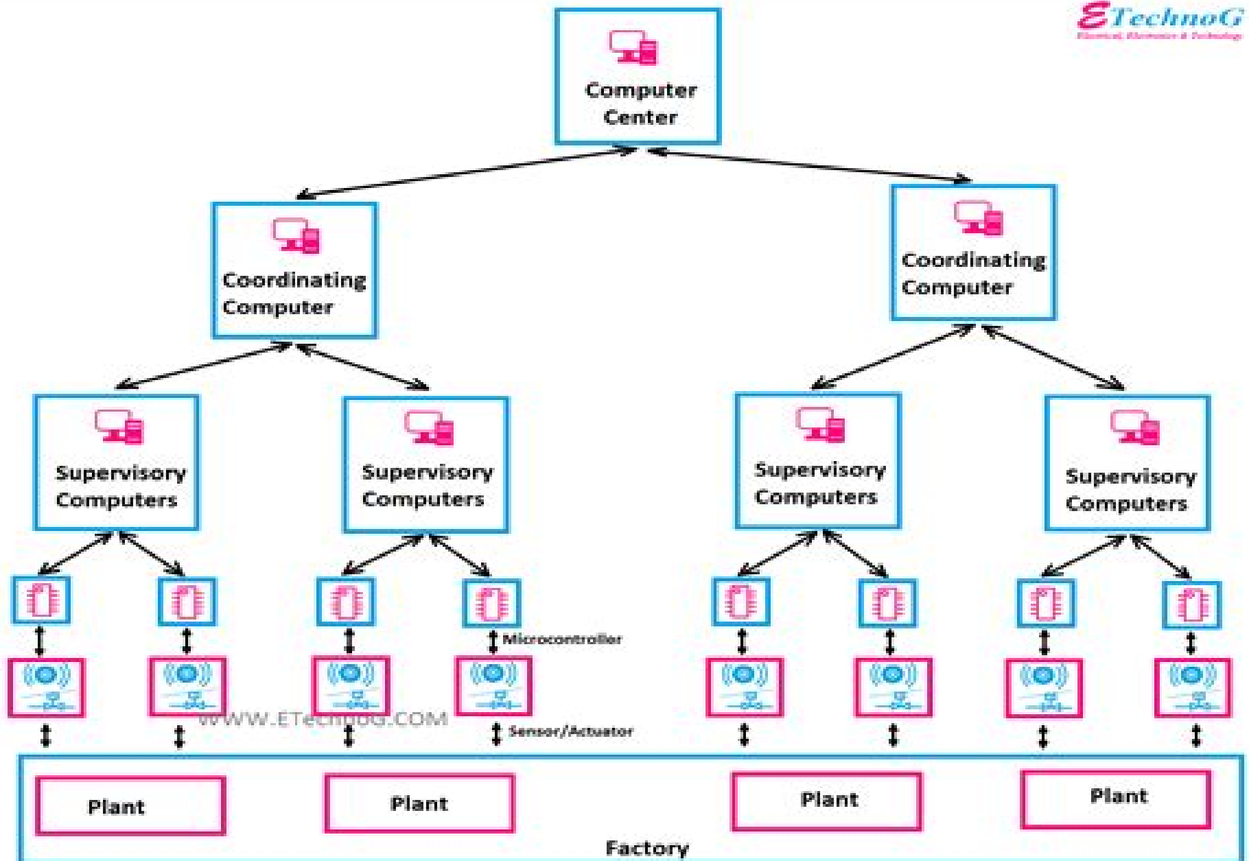
Distributed Control System(DCS) Block Diagram
