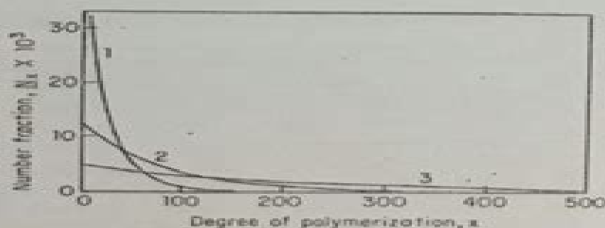
Fig. 2-11 Number fraction distribution curve for linear polymerization. Curve 1: p = 0.9600 ; curve 2: p = 0.9875 ; curve 3: p = 0.9950 . After [52] (by permission of Interscience, Ltd., London).
