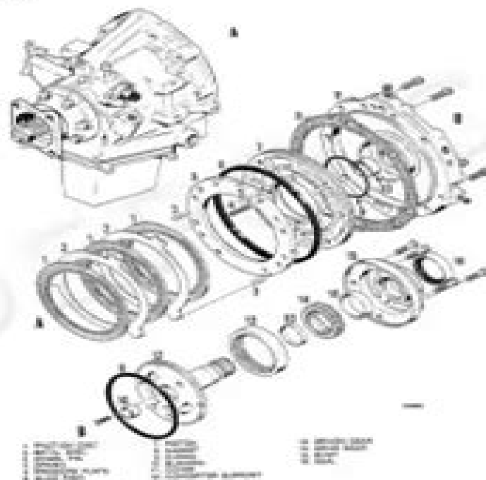
Figure 4-1: Exploded Pump and Reverse Clutch
