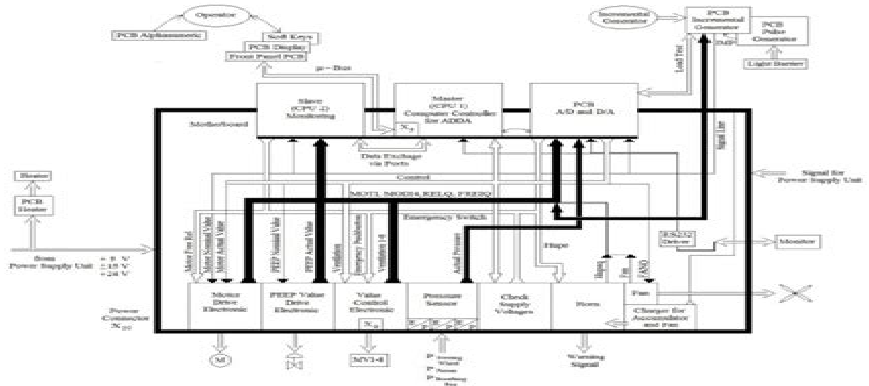
Figure 1 - Block Diagram of Data Transfer for Dräger Cato
