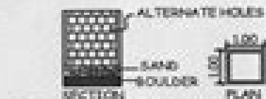
DETAILS OF RAIN WATER HARVESTING TANK
