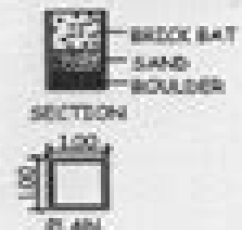
DETAILS OF SOAK PIT
