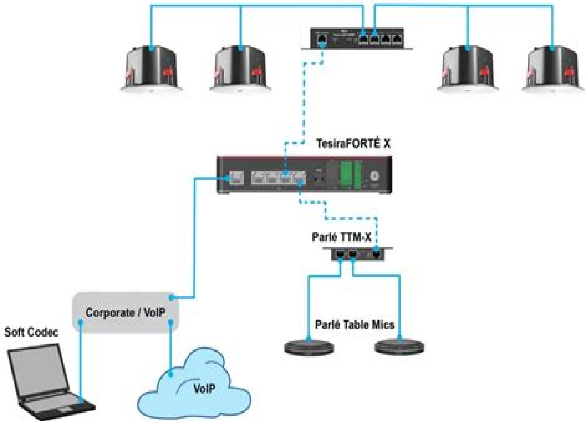
AMP-450BP with 4 Speakers
