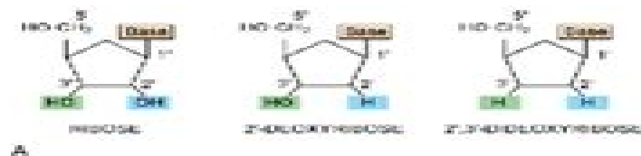
STRUCTURES OF RIBOSE, DEOXYRIBOSE, AND DIDEOXYRIBOSE
