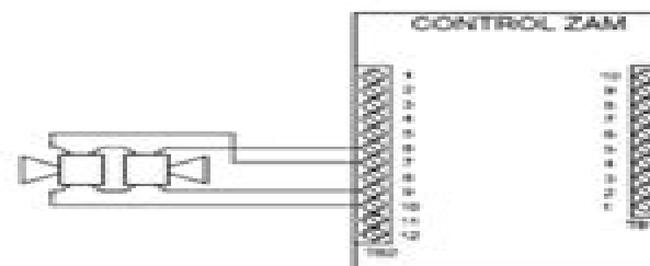
Figure 3. Class A Signal ZAM, NAC Wiring
