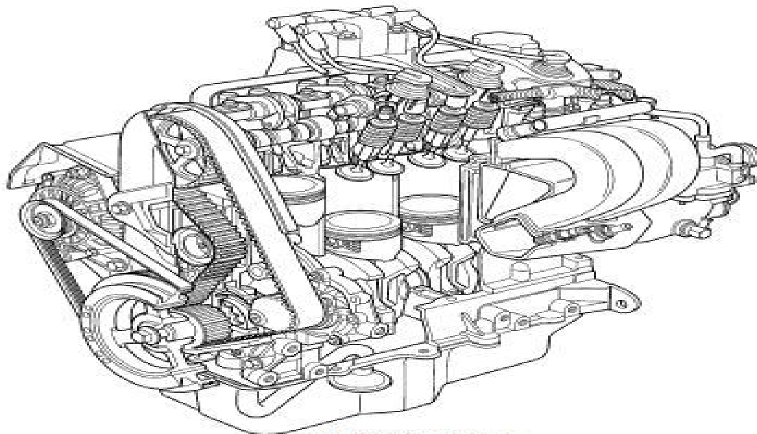
Fig. 1 2.0L SOHC Engine
