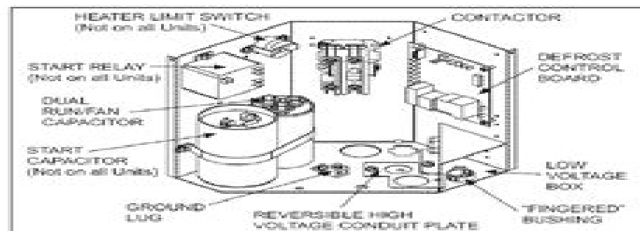
FIGURE 7: Outdoor Unit Control Box
