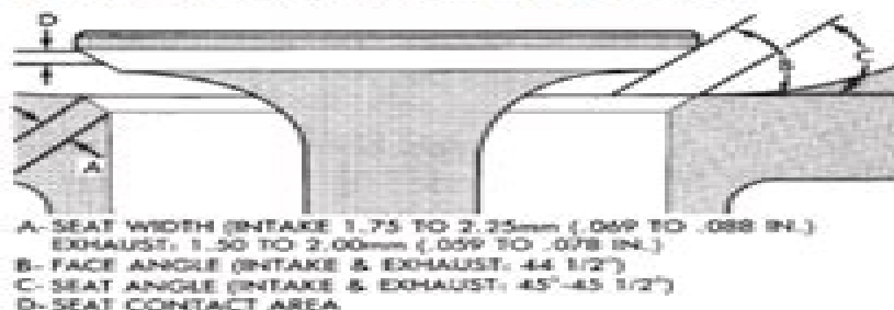
Fig. 20 Valve Seats
