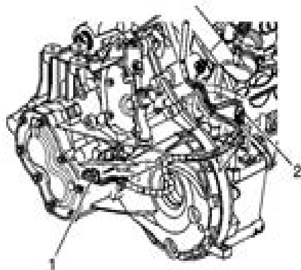
Fig. 80: Locating Backup Light Connector & ABS Connector Courtesy of GENERAL MOTORS CORP.
