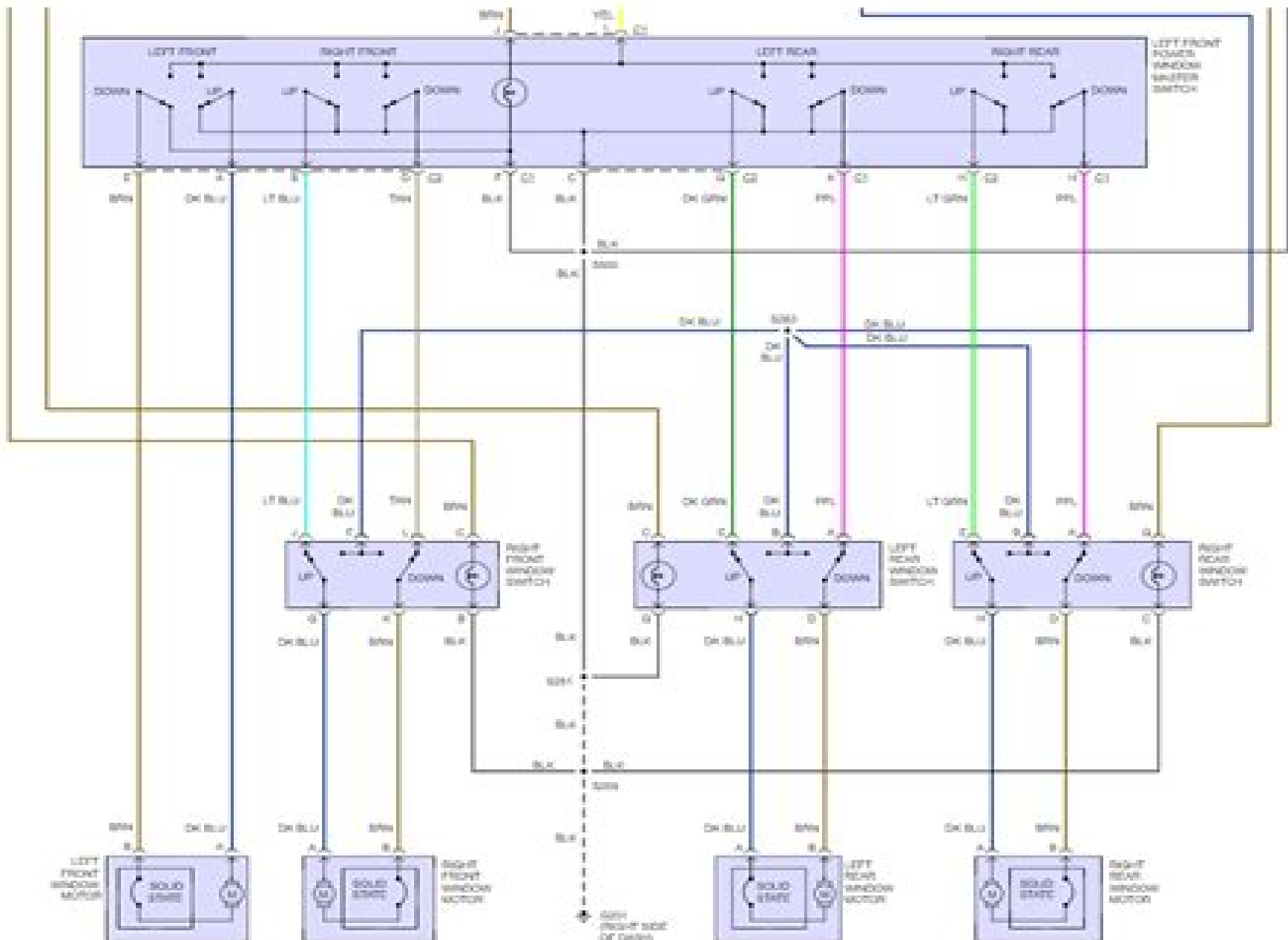
Fig 2: Power Window Circuit, 4 Door
