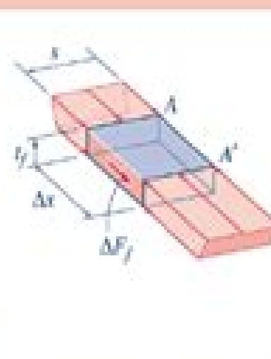
(c) A free-body diagram for determining flange shear flow.
