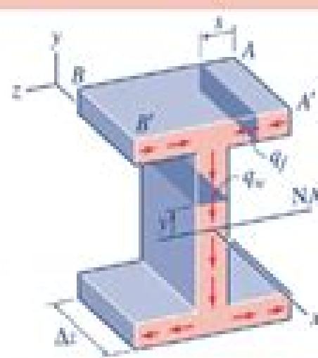
(b) Cutting planes used to determine the flange shear flow q_f and the web shear flow q_w .
