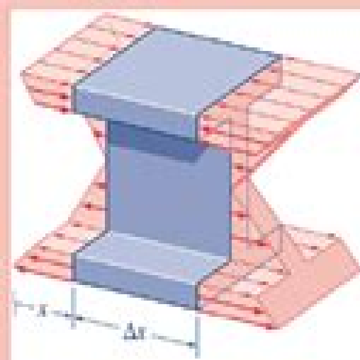
(a) A beam segment showing flexural stresses due to M(x) and due to M(x + \Delta x) .
