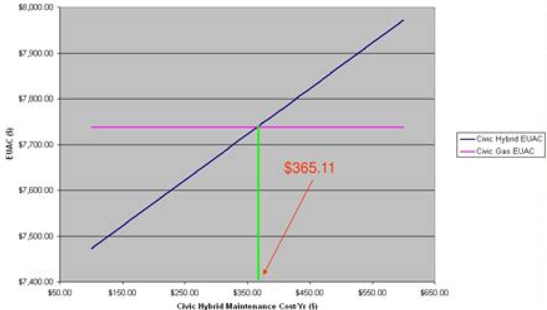
Sensitivity and Breakeven Analysis: EUAC vs. Civic Hybrid Maintenance Cost/Yr
