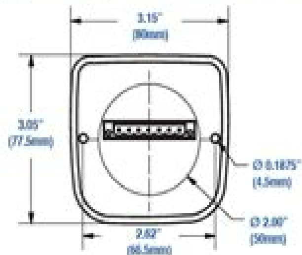
Mounting and wiring terminal hole sizes and location.
