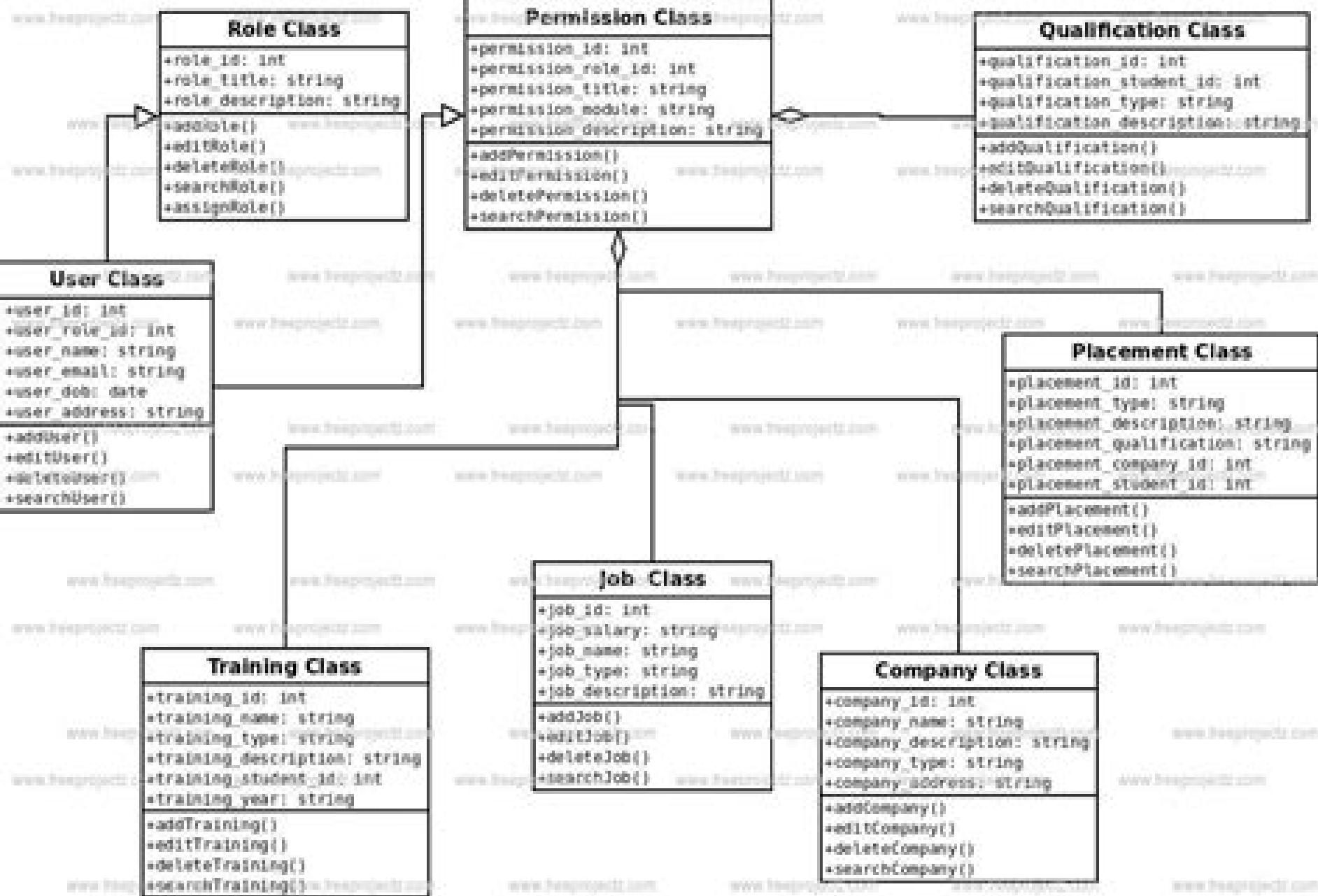
Class Diagram of Training and Placement Management System
