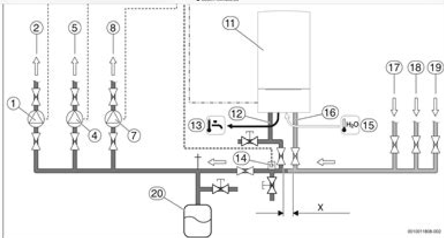
Fig. 8 Piping
