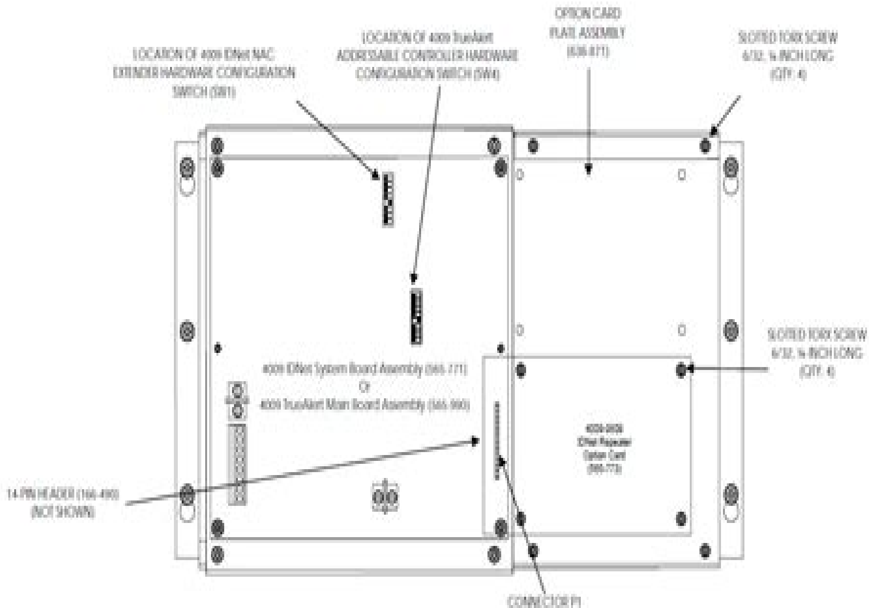
Figure 3. IDNet Repeater Option Card Installation
