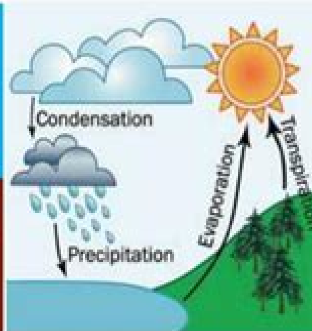
Water Cycle
