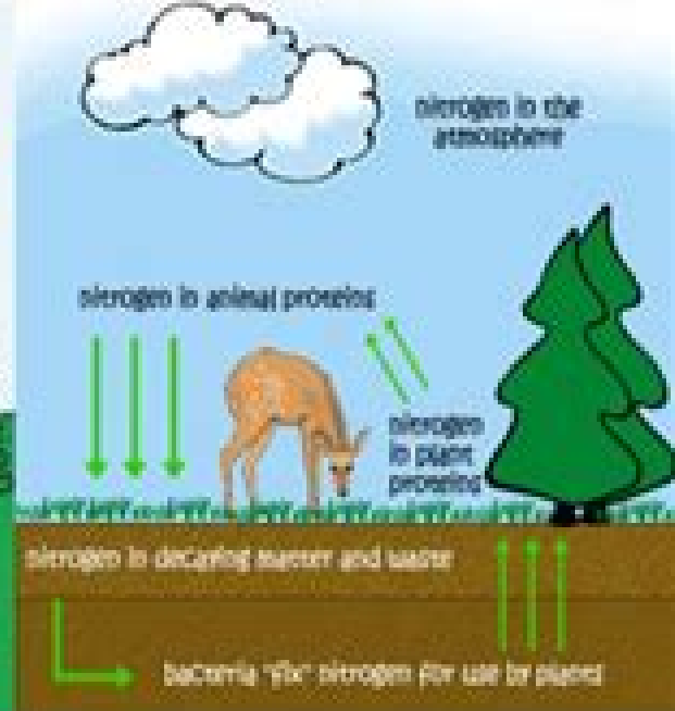
Nitrogen Cycle
