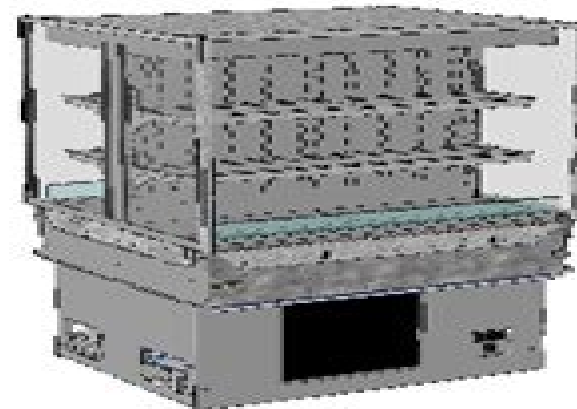
Dual Access - "V2" Dual Access Model With Perforated Back-To-Back Rear Panels (Cladding Removed For Illustrative Purposes Only)
