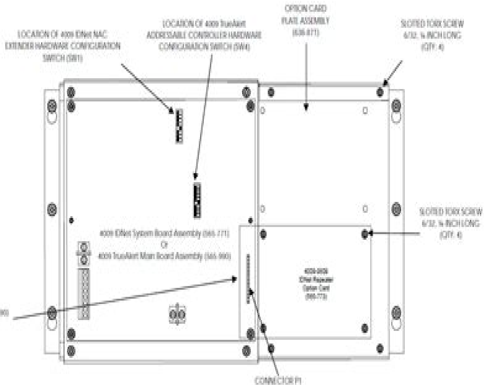
Figure 3. IDNet Repeater Option Card Installation
