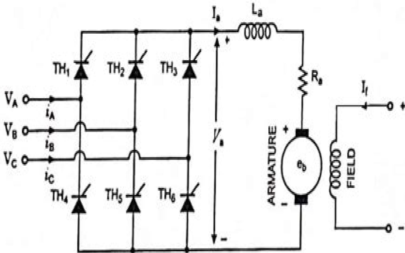
Fig. 27.21 Three-Phase Fullconverter Supplying Separately Excited DC Motor
