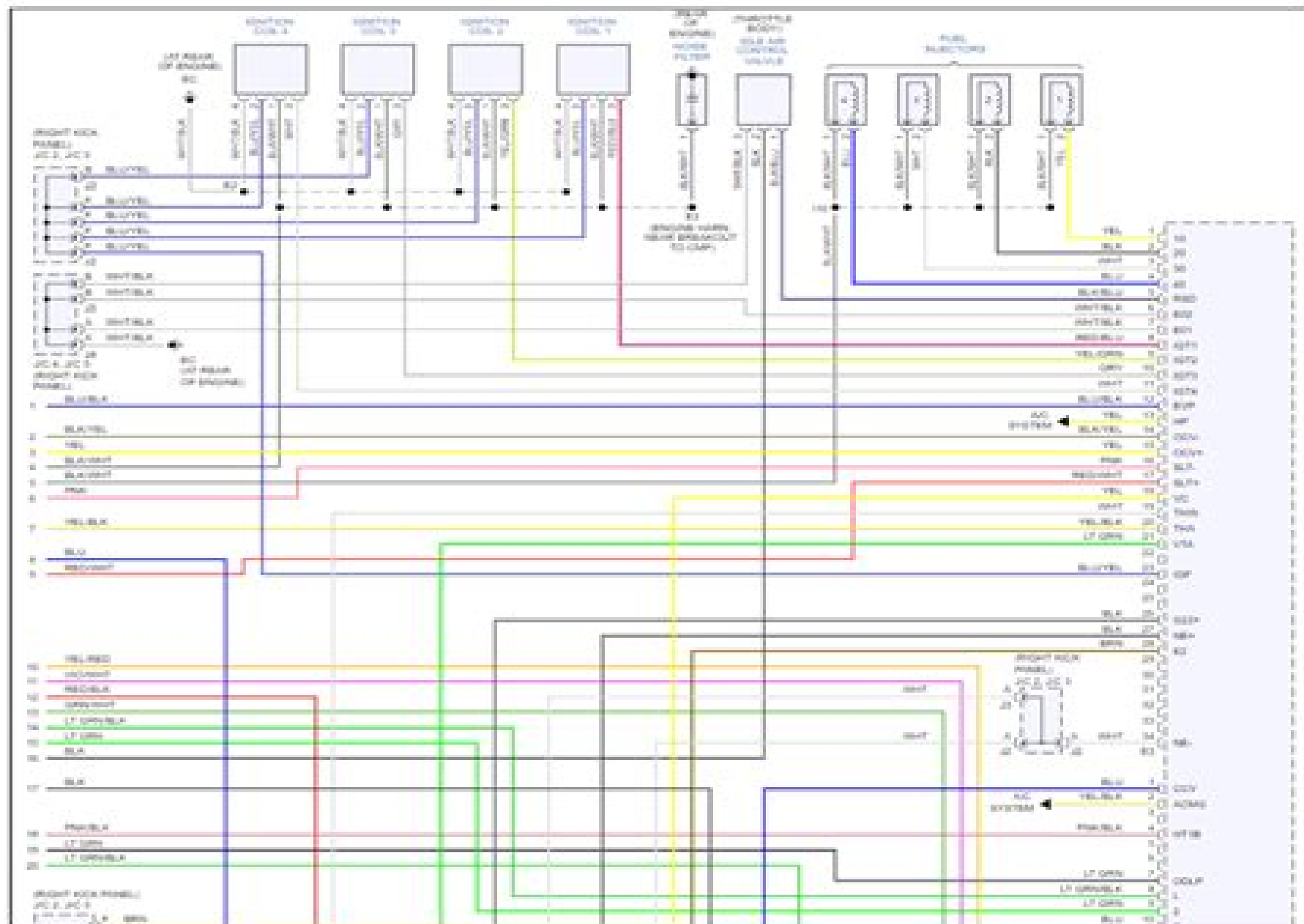
Fig 3: 1.8L, Engine Performance Circuit (3 of 3)
