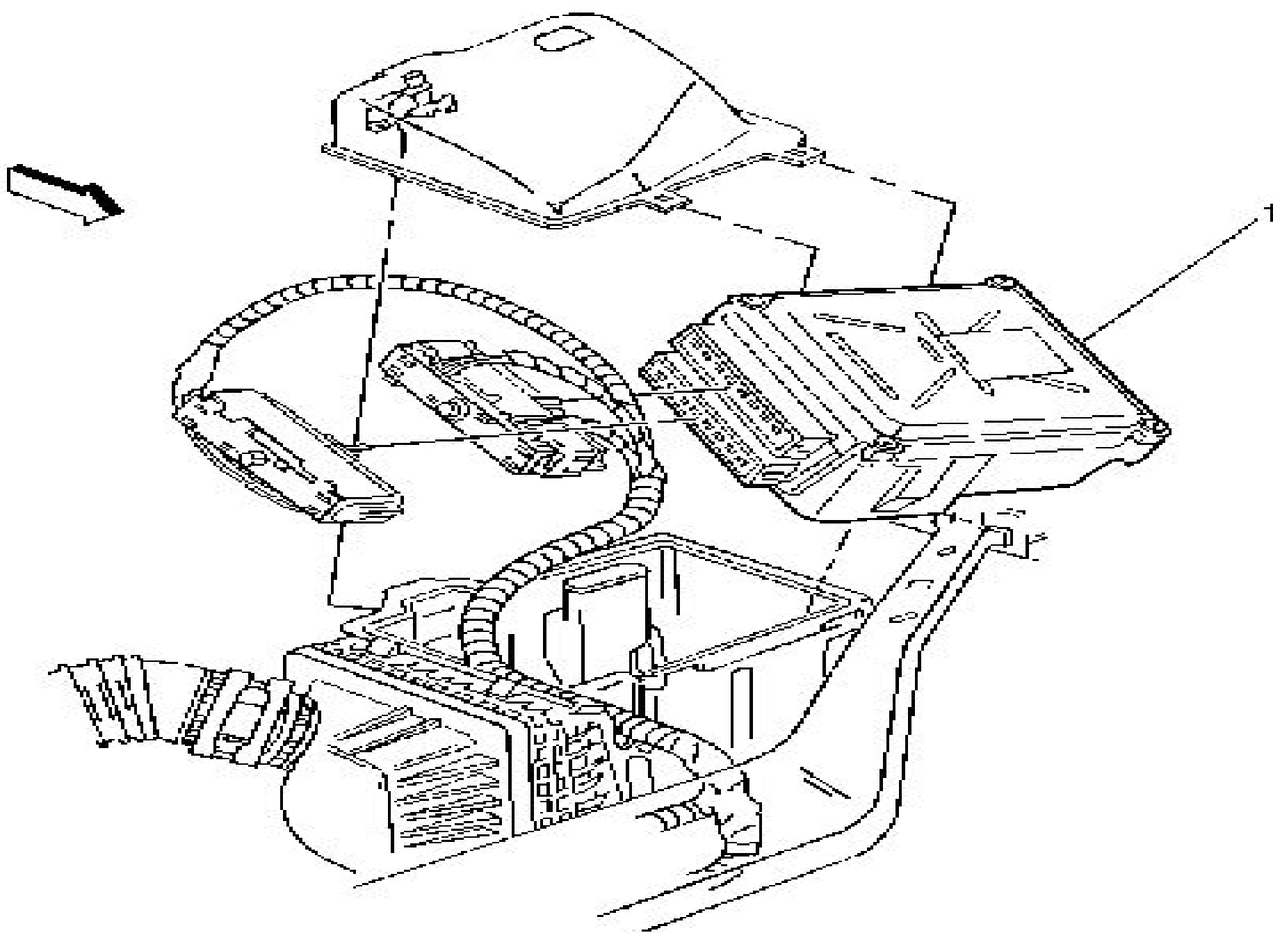
(1) Powertrain Control Module
