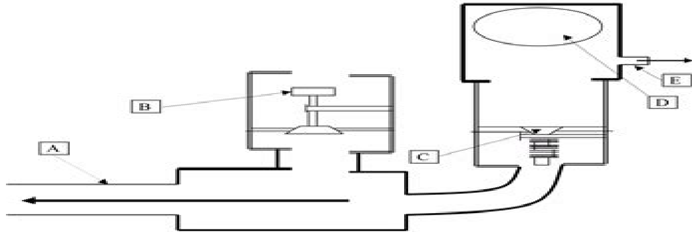
Figure 3. Hydraulic Ram Sequence III
