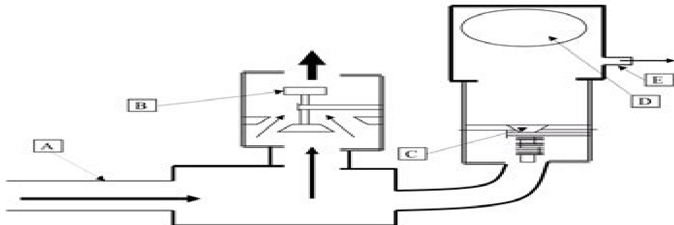
Figure 4. Hydraulic Ram Sequence IV
