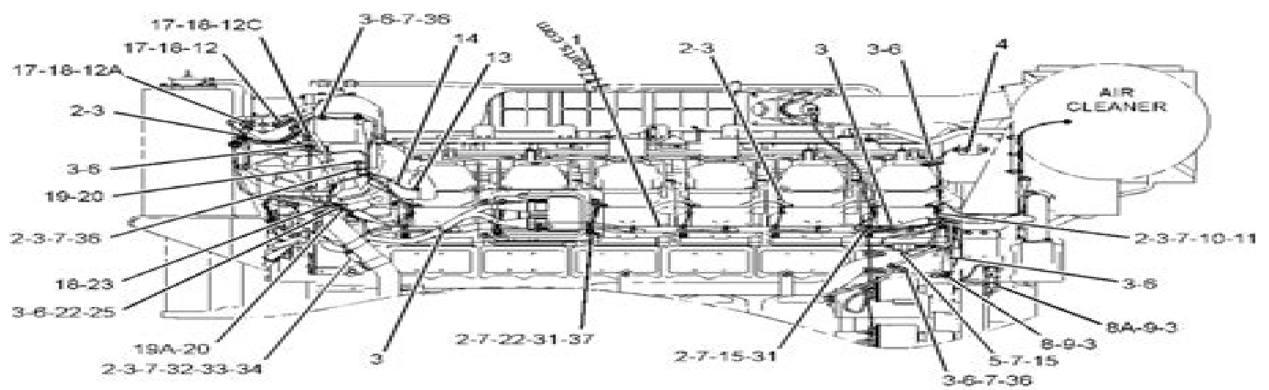
LEFT SIDE VIEW OF ENGINE
