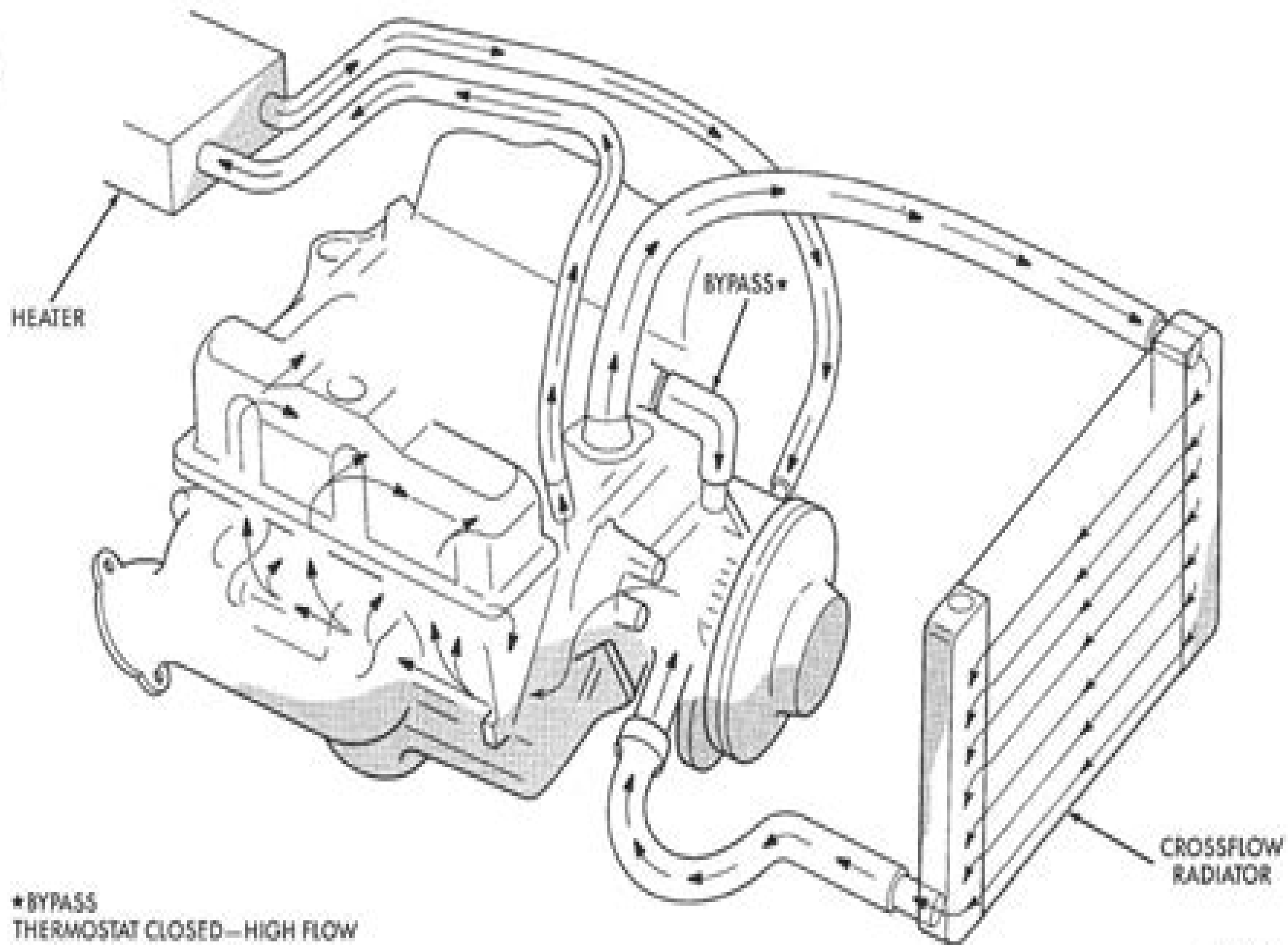
Fig. 2 Engine Cooling System—5.2/5.9L Engine—Typical
