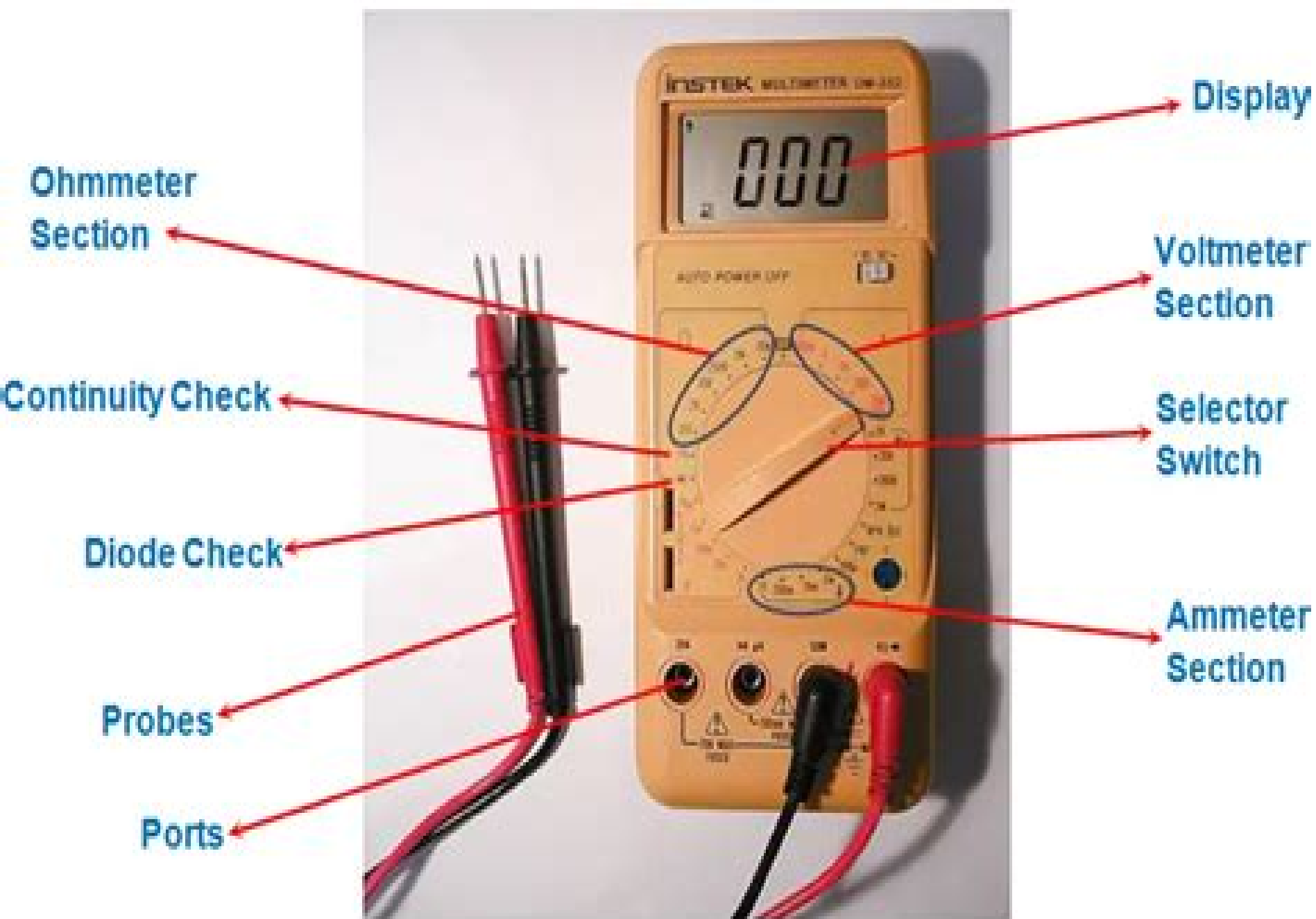
Figure 1 A Typical Digital Multimeter
