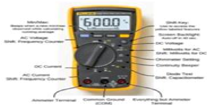
Figure 1: Fluke 115 Multimeter
