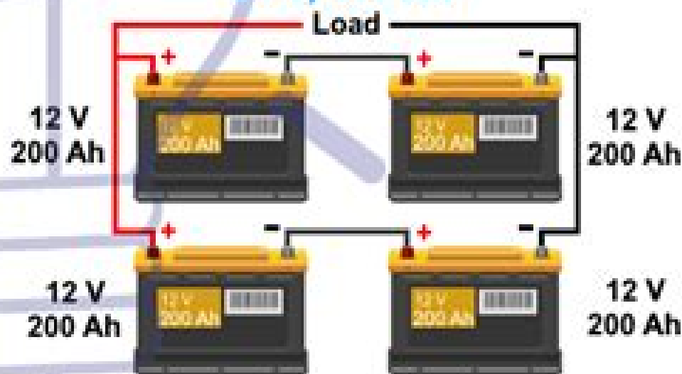
2 Parallel Sets of 2 Batteries in Series (Series-Parallel Connection)
