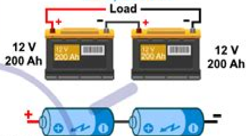
2 Batteries in Series
