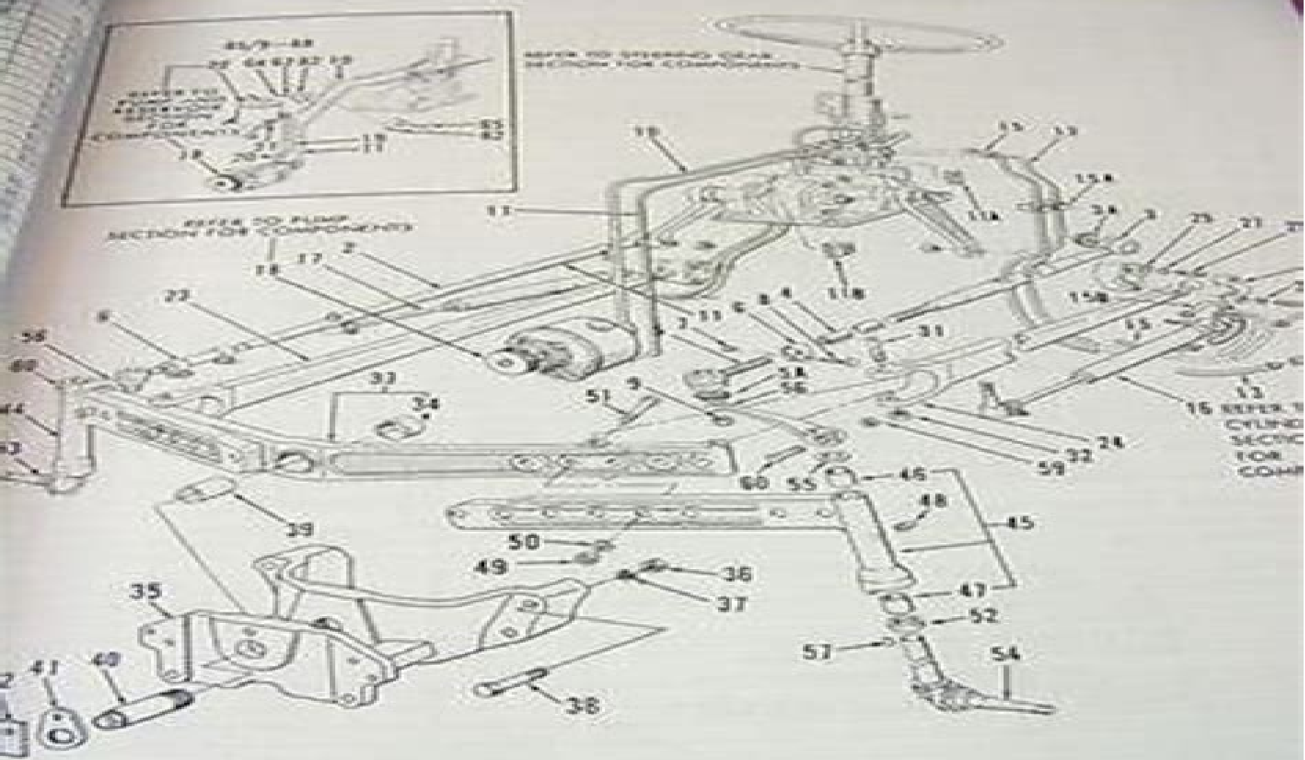
FIG. 342 - FRONT AXLE, POWER STEERING & RELATED PARTS (2000 & 3000) Supplement
