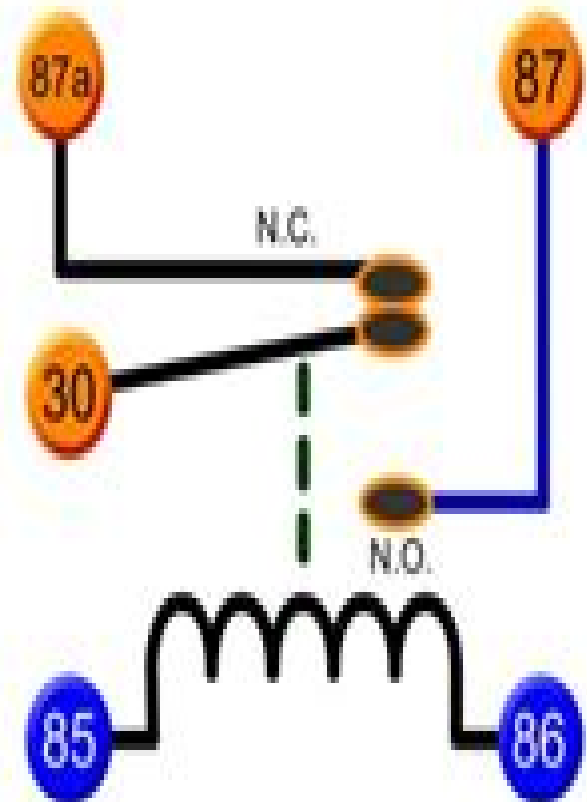
Wiring Diagram
